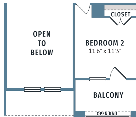
BELLE 2
