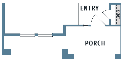
BELLE 2
