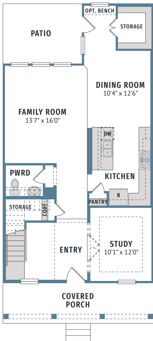
MAIN FLOOR
