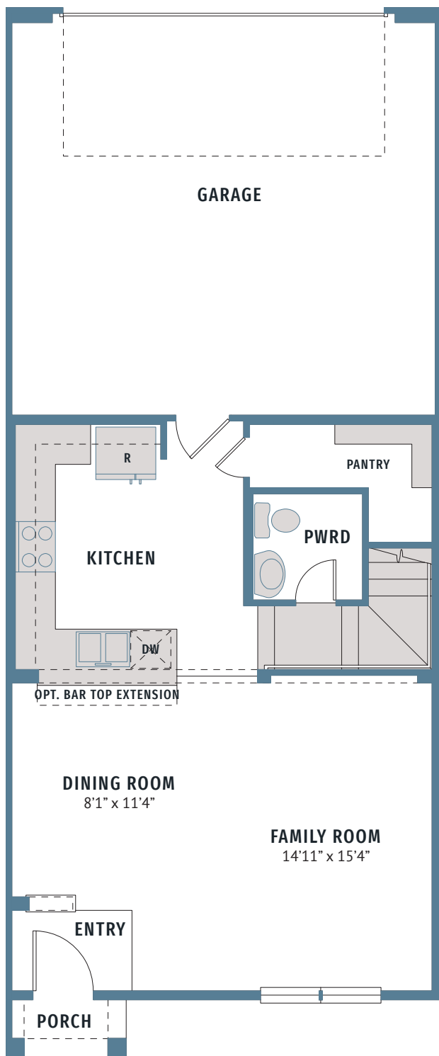
MAIN FLOOR
