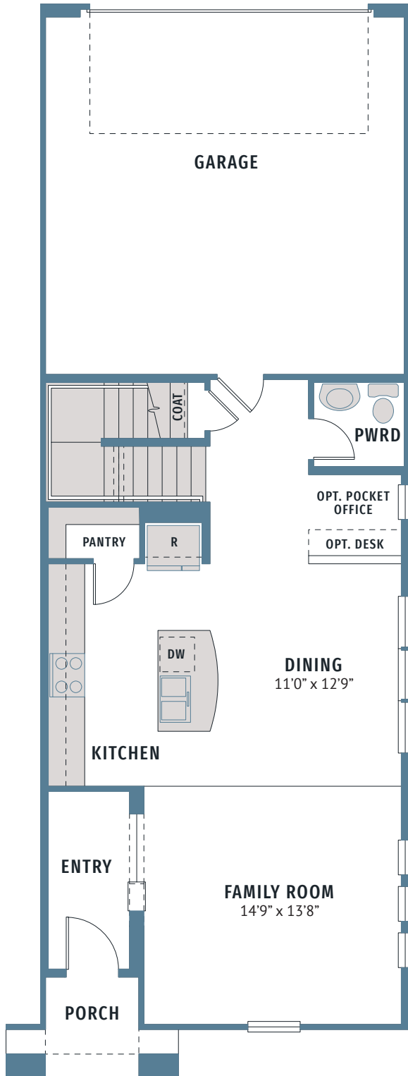
MAIN FLOOR
