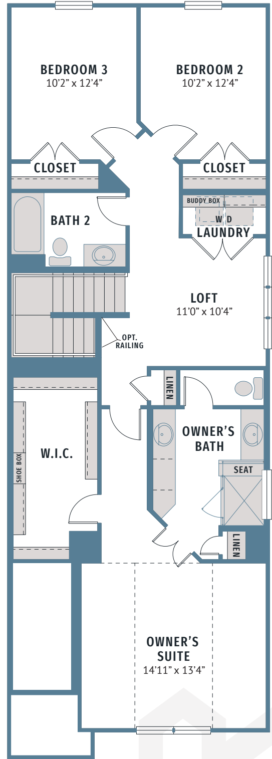
UPPER FLOOR
