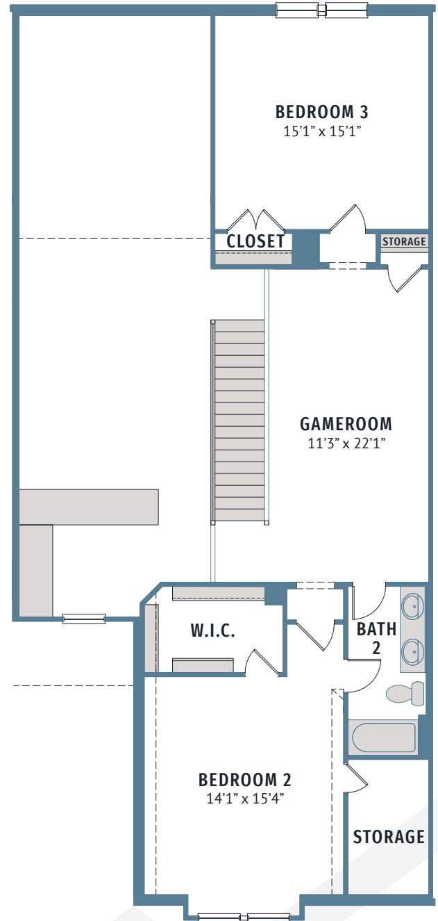
UPPER FLOOR
