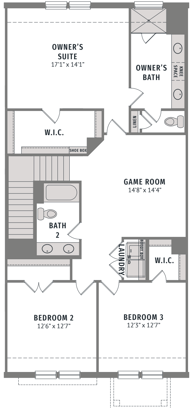
UPPER FLOOR - GEORGIAN
