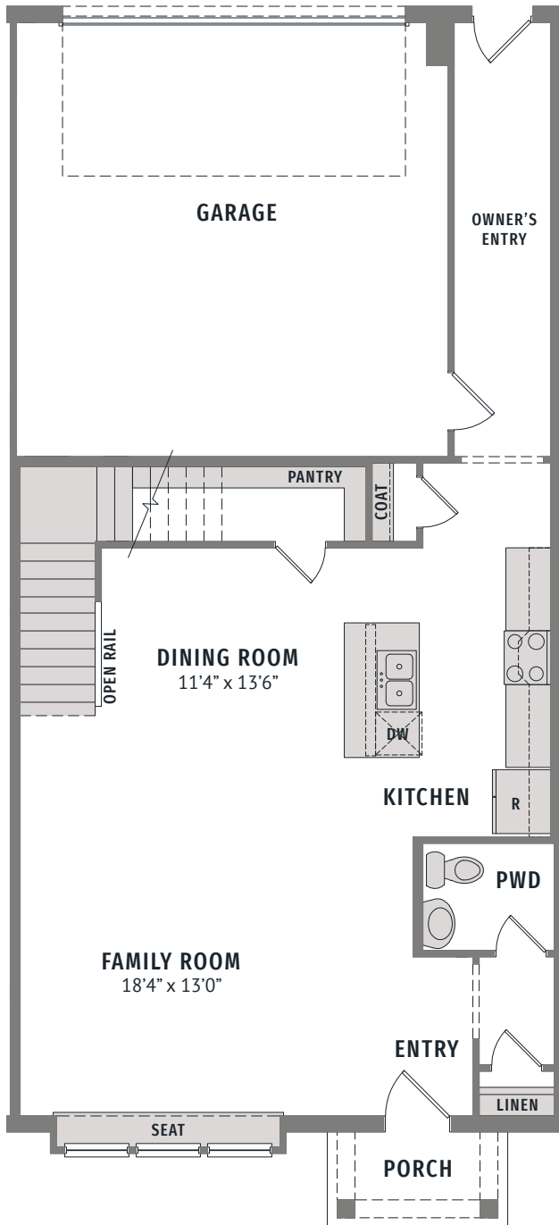
MAIN FLOOR - GEORGIAN
