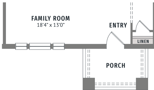
MAIN FLOOR - CRAFTSMAN
