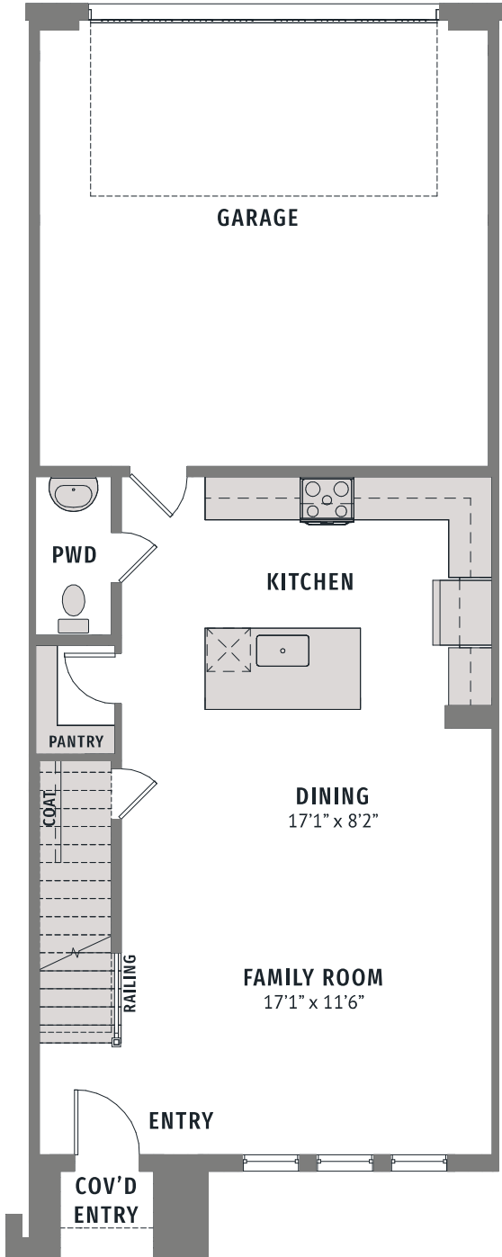
MAIN FLOOR
